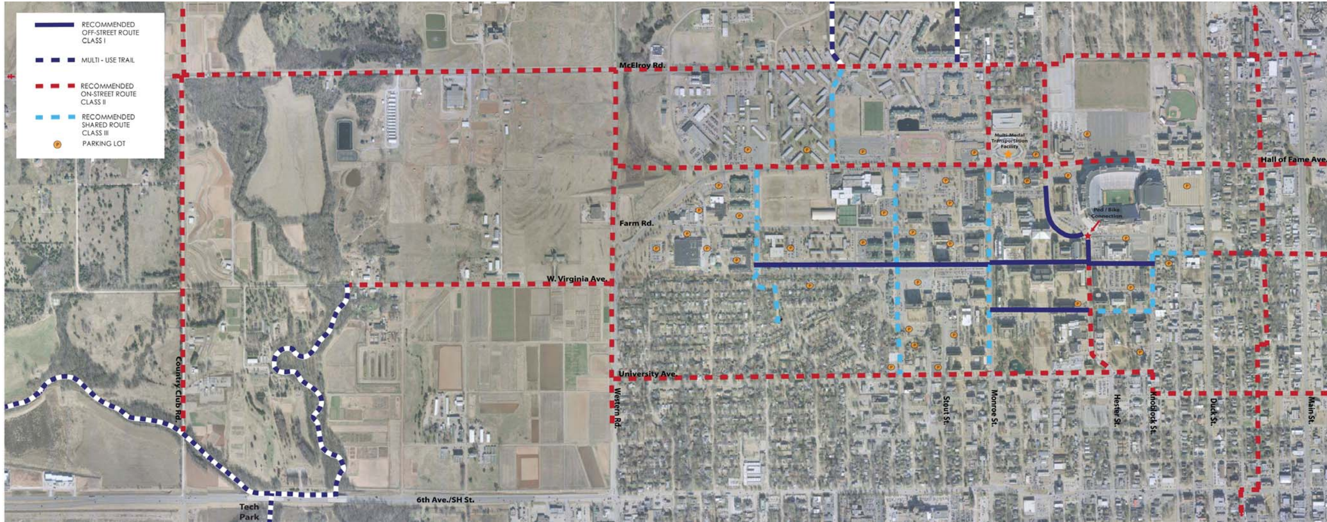
FIGURE 6.3 RECOMMENDED CAMPUS / COMMUNITY BICYCLE CONNECTIVITY
