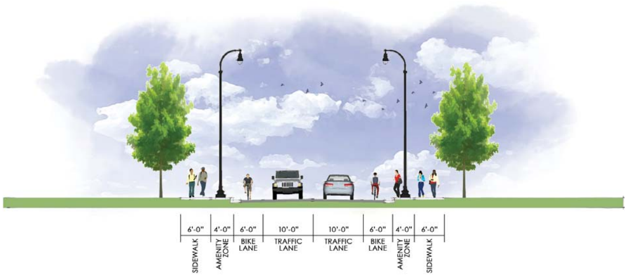
Figure 3.18 -Typical Access Corridor Section with Attached Sidewalks
