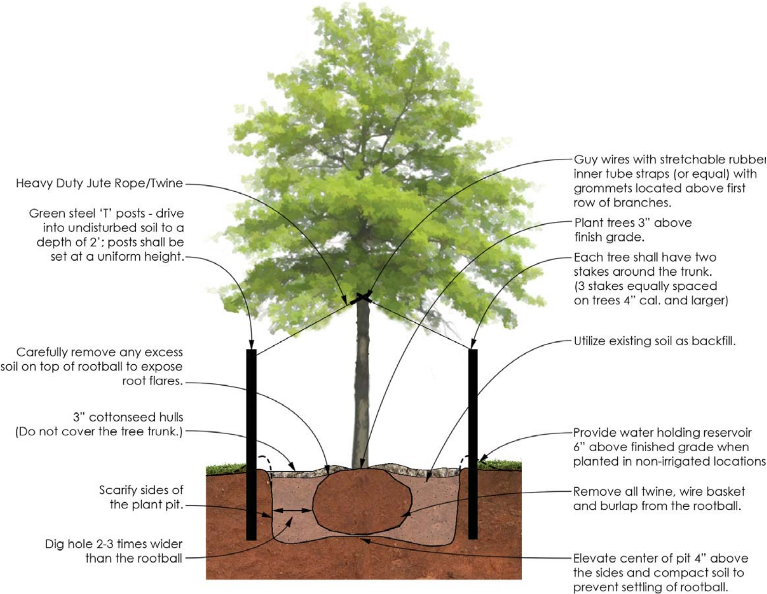
Typical Tree Planting Detail
