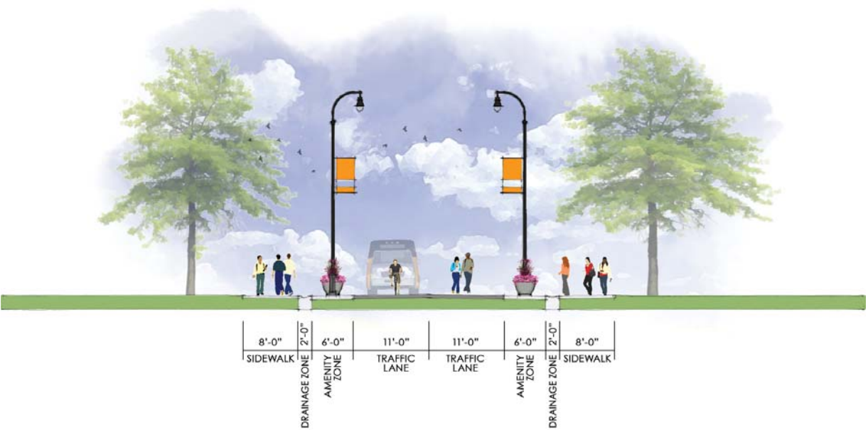
Figure 3.10 - Recommended Monroe and Hester Street Section
