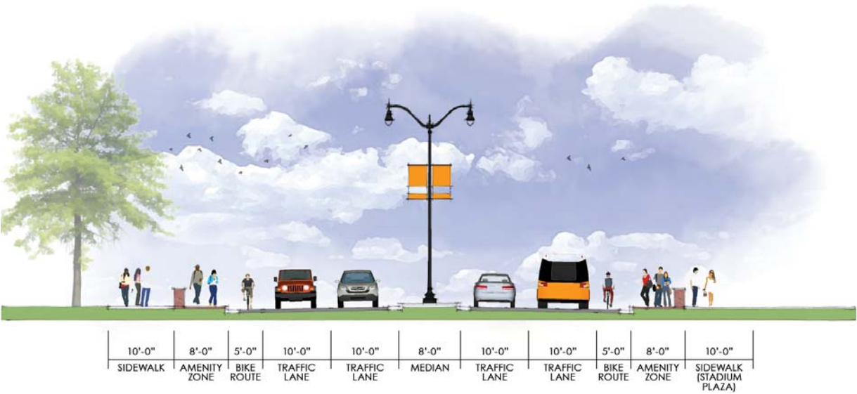
Figure 3.2 - Recommended Hall of Fame Avenue Section (between Duck Street and Monroe Street) (Note: This section of Hall of Fame Avenue has recently been reconstructed. The recommended lane widths shown for vehicular traffic and bicycles work with the existing curb to curb street width.)
