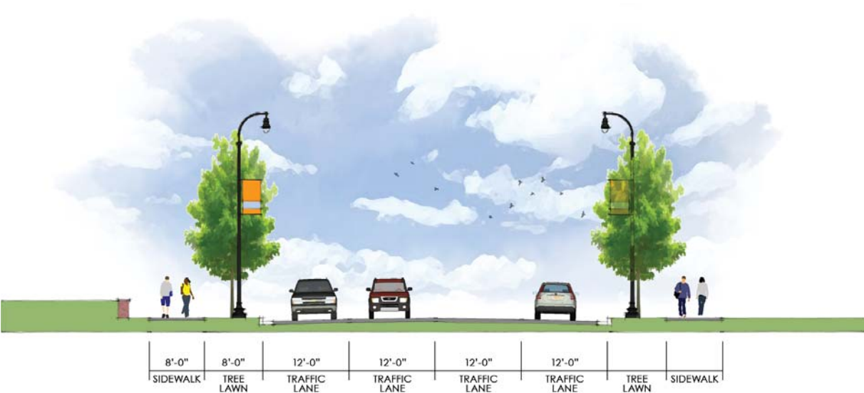
Figure 3.5 - Recommended Duck Street Section
