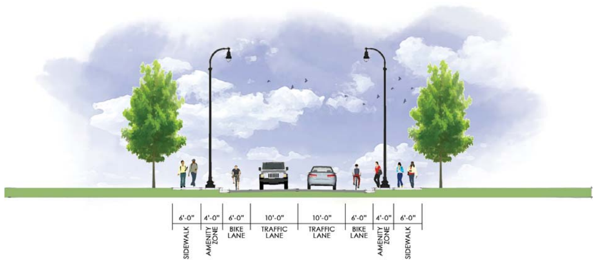
Figure 3.9 - Recommended Access Street with Attached Sidewalks
