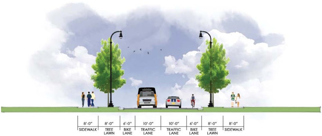
Figure 3.8 - Recommended Access Street with Detached Sidewalks
