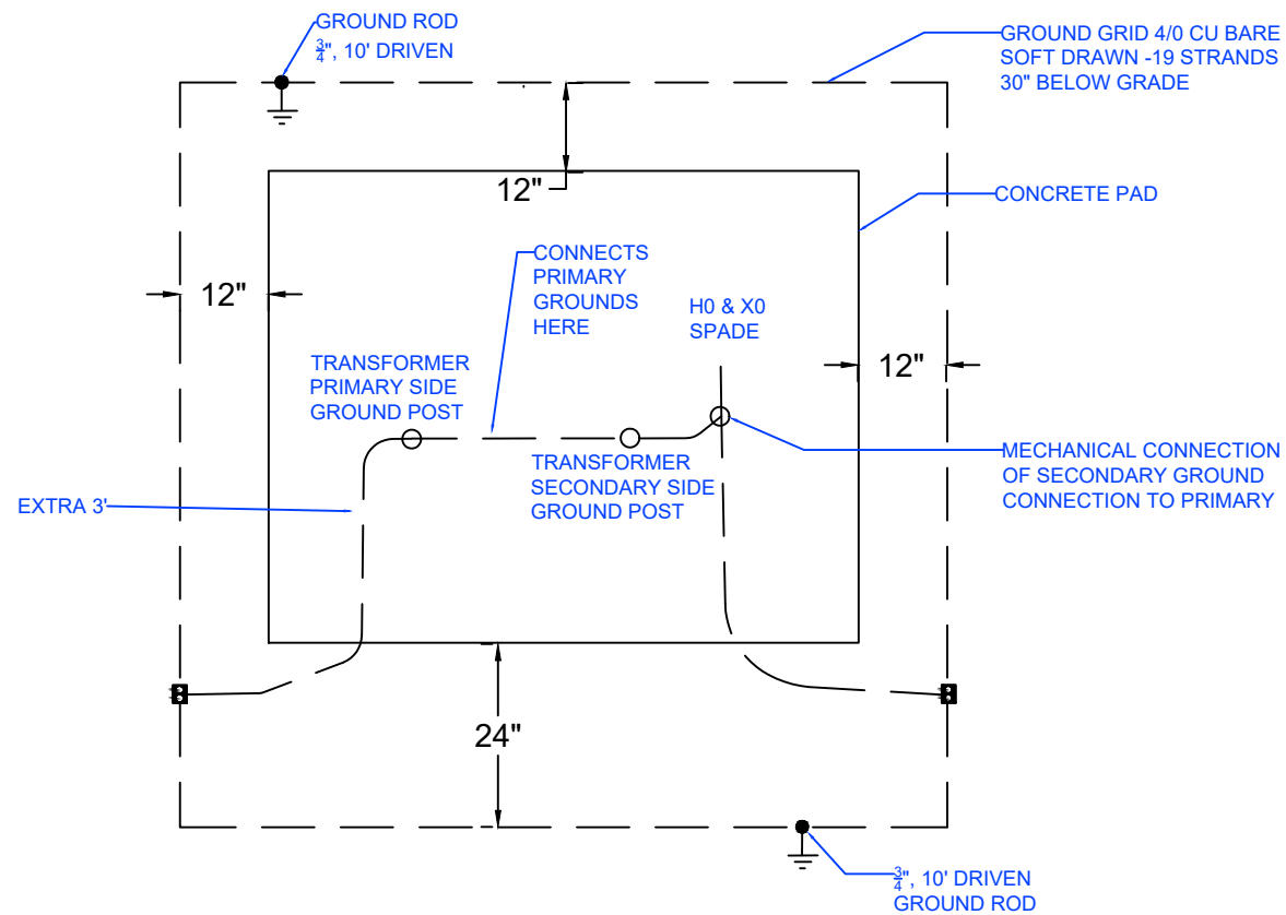
1 TRANSFORMER GROUNDING NTS
